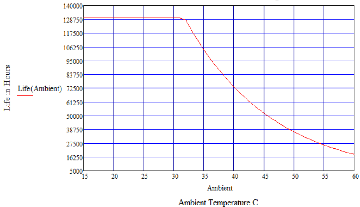
LD40W480 Estimated Life Full Load @ 347Vac
