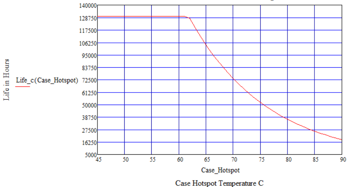
LD40W480 Estimated Life Full Load @ 347Vac
