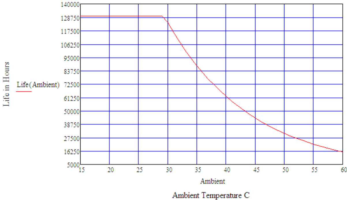
LDHL40W Estimated Life Full Load @ 120Vac
