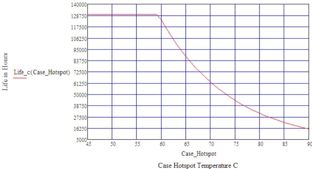
LDHL40W Estimated Life Full Load @ 120Vac
