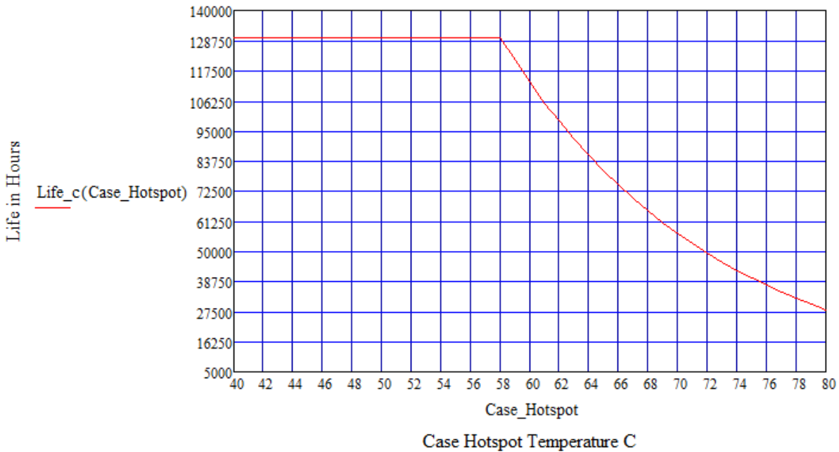
LD17W Estimated Life Full Load @ 120Vac
