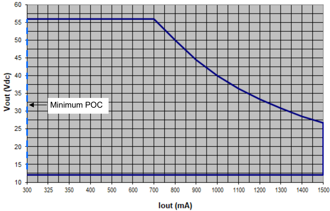
POWER OPERATING WINDOW Vout (Vdc) vs. Output Current (mA)
