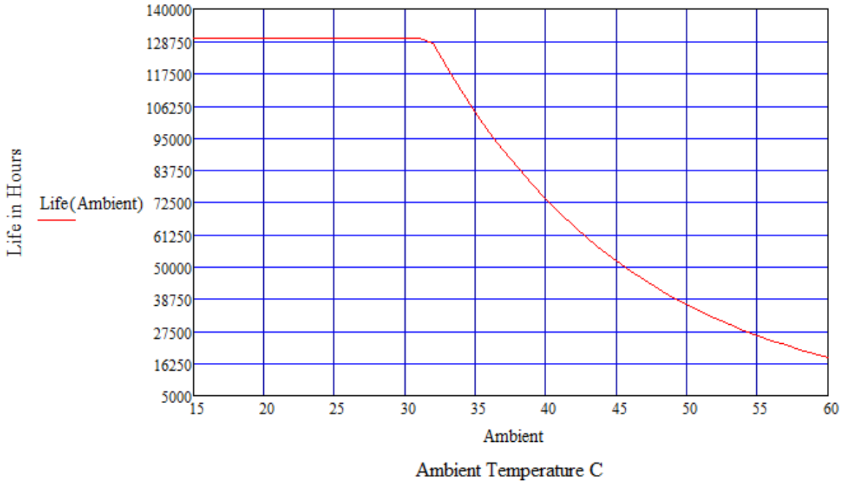
LP40W Estimated Life Full Load @ 120Vac
