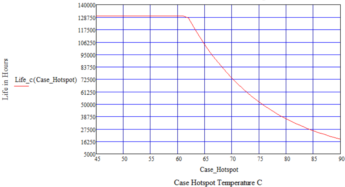
LP40W Estimated Life Full Load @ 120Vac
