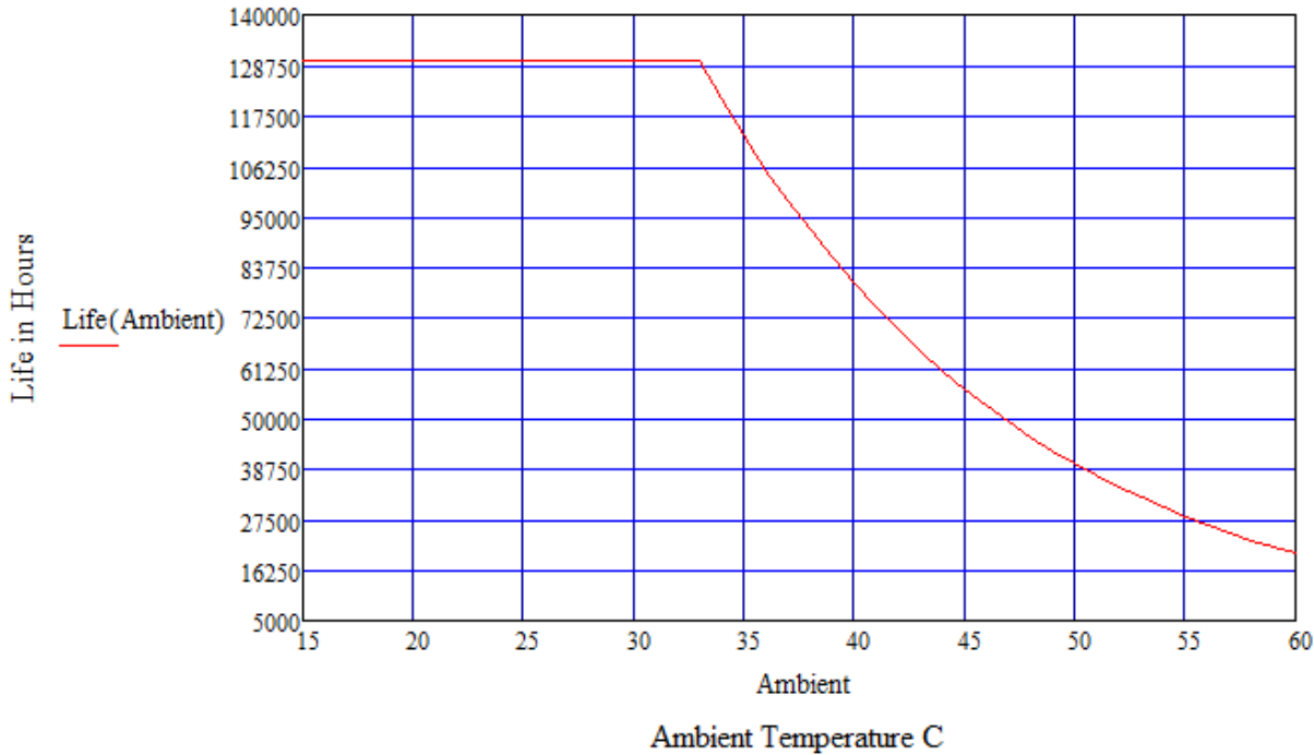
LP50WT5 Estimated Life Full Load @ 120Vac
