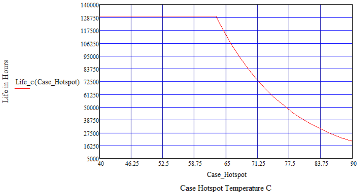
LP50WT5 Estimated Life Full Load @ 120Vac
