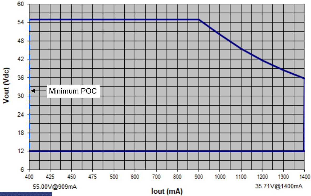
LP50WT5-55-PC1400-RD OPERATING WINDOW Vout (Vdc) vs. Output Current (mA)
