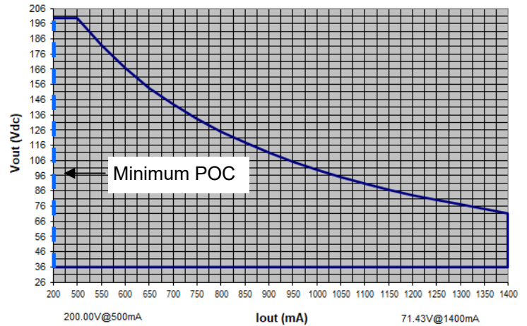
LPF100W-200-PC1400-RD OPERATING WINDOW Vout (Vdc) vs. Output Current (mA)
