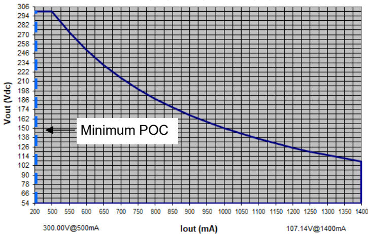
LPF150W-300-PC1400-RD OPERATING WINDOW Vout (Vdc) vs. Output Current (mA)
