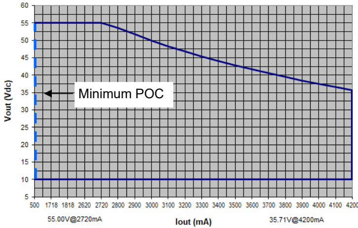
LPF150W-55-PC4200-RD OPERATING WINDOW Vout (Vdc) vs. Output Current (mA)
