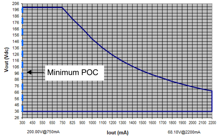
LPF150W-200-PC2200-RD OPERATING WINDOW Vout (Vdc) vs. Output Current (mA)
