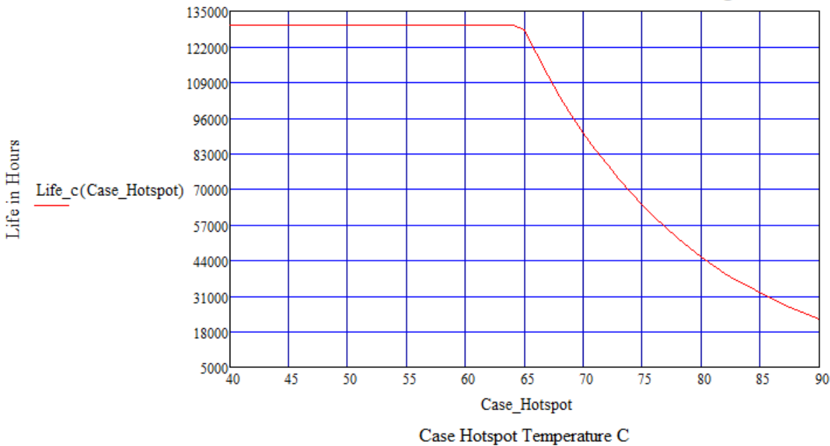
LPF150W-XX-PCXXXX-RD Estimated Life Full Load @ 120Vac
