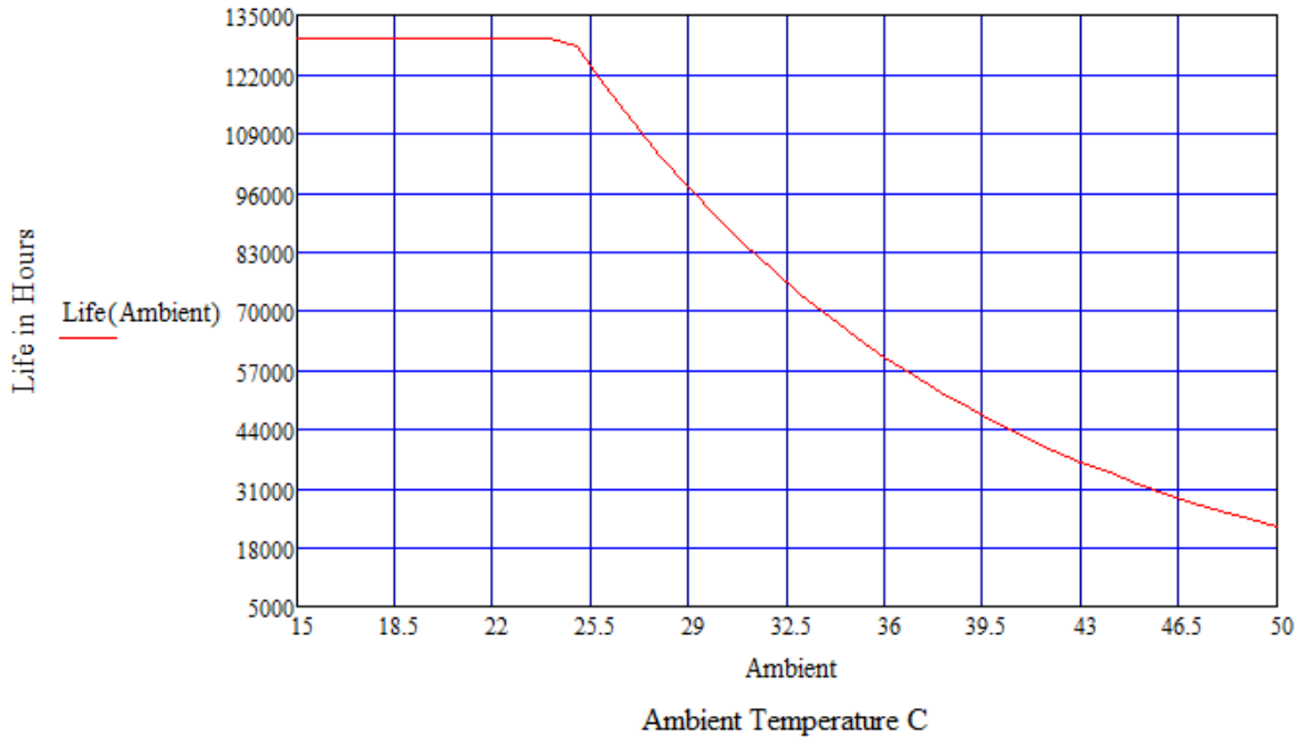
LPF150W-XX-PCXXXX-RD Estimated Life Full Load @ 120Vac
