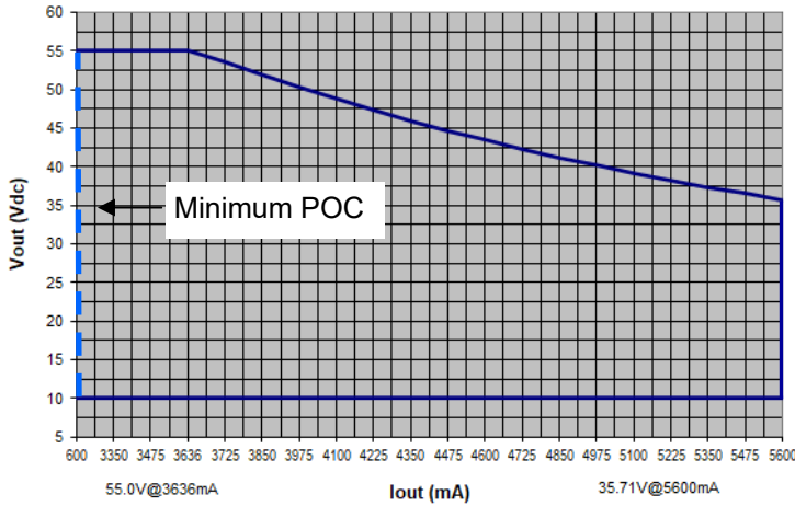
LP200W-55-PC5600-RD OPERATING WINDOW Vout (Vdc) vs. Output Current (mA)
