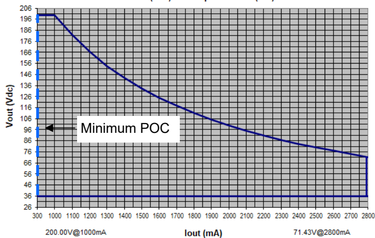
LP200W-200-PC2800-RD OPERATING WINDOW Vout (Vdc) vs. Output Current (mA)
