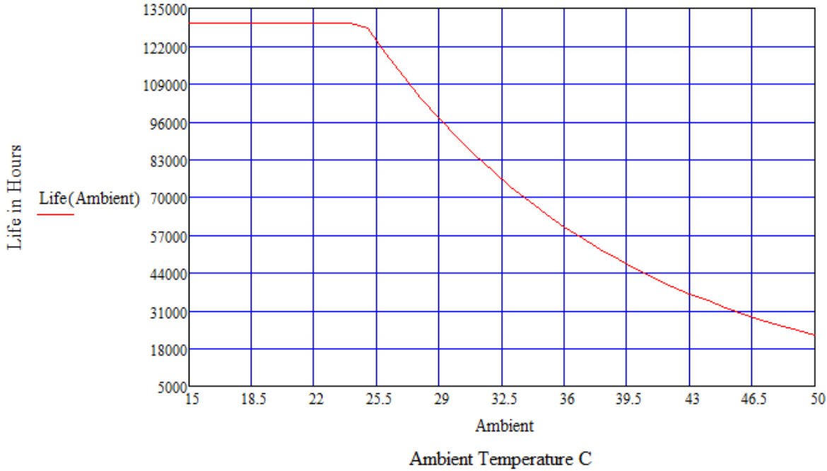
LPF200W-XX-PCXXXX-RD Estimated Life Full Load @ 120Vac
