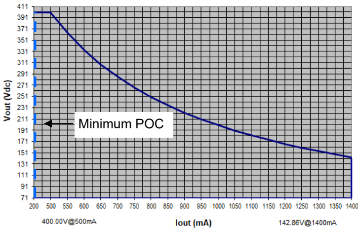
LP200W-400-PC1400-RD OPERATING WINDOW Vout (Vdc) vs. Output Current (mA)
