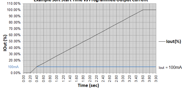
Example Soft Start Time vs Programmed Output Current
