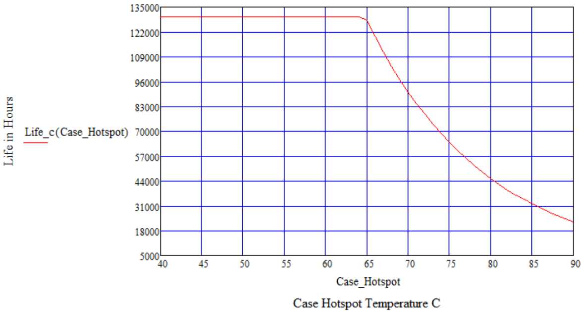
LPF200W-XX-PCXXXX-RD Estimated Life Full Load @ 120Vac
