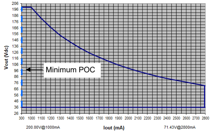
LP200W-200-PC2800-RD OPERATING WINDOW Vout (Vdc) vs. Output Current (mA)
