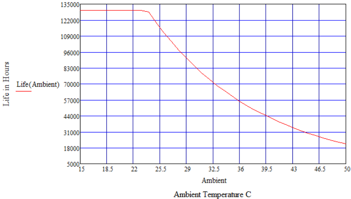
LPF240W-XX-PCXXXX-RD Estimated Life Full Load @ 120Vac
