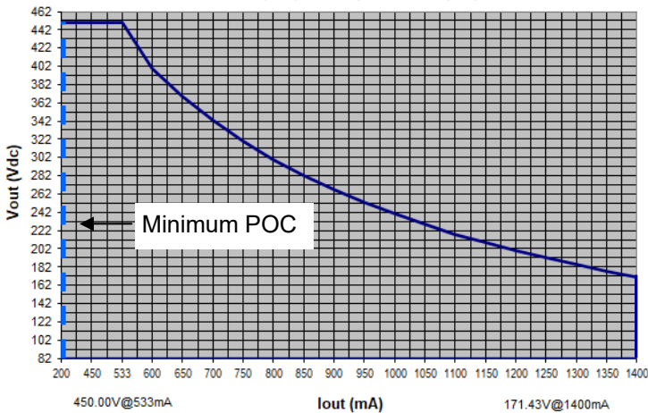
LPF240W-450-PC1400-RD OPERATING WINDOW Vout (Vdc) vs. Output Current (mA)
