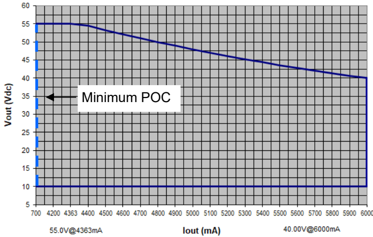
LPF240W-55-PC6000-RD OPERATING WINDOW Vout (Vdc) vs. Output Current (mA)
