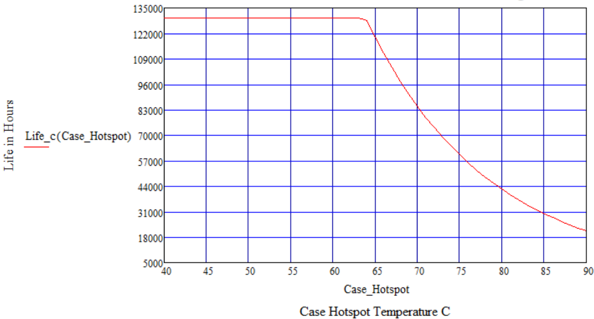
LPF240W-XX-PCXXXX-RD Estimated Life Full Load @ 120Vac
