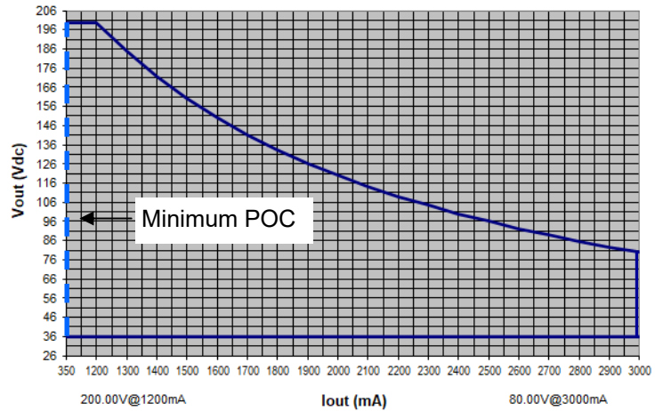
LPF240W-200-PC3000-RD OPERATING WINDOW Vout (Vdc) vs. Output Current (mA)
