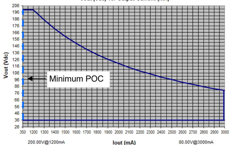
LPF240W-200-PC3000-RD OPERATING WINDOW Vout (Vdc) vs. Output Current (mA)
