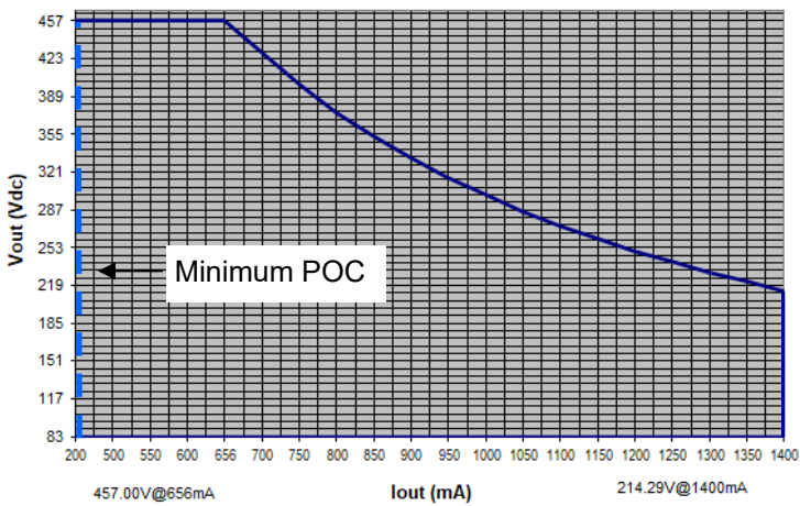
LPF300W-457-PC1400-RD OPERATING WINDOW Vout (Vdc) vs. Output Current (mA)
