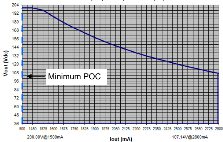
LPF300W-200-PC2800-RD OPERATING WINDOW Vout (Vdc) vs. Output Current (mA)
