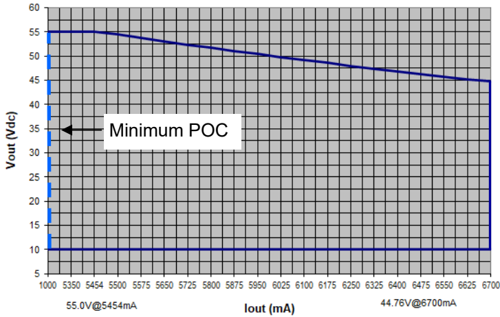
LPF300W-55-PC6700-RD OPERATING WINDOW Vout (Vdc) vs. Output Current (mA)
