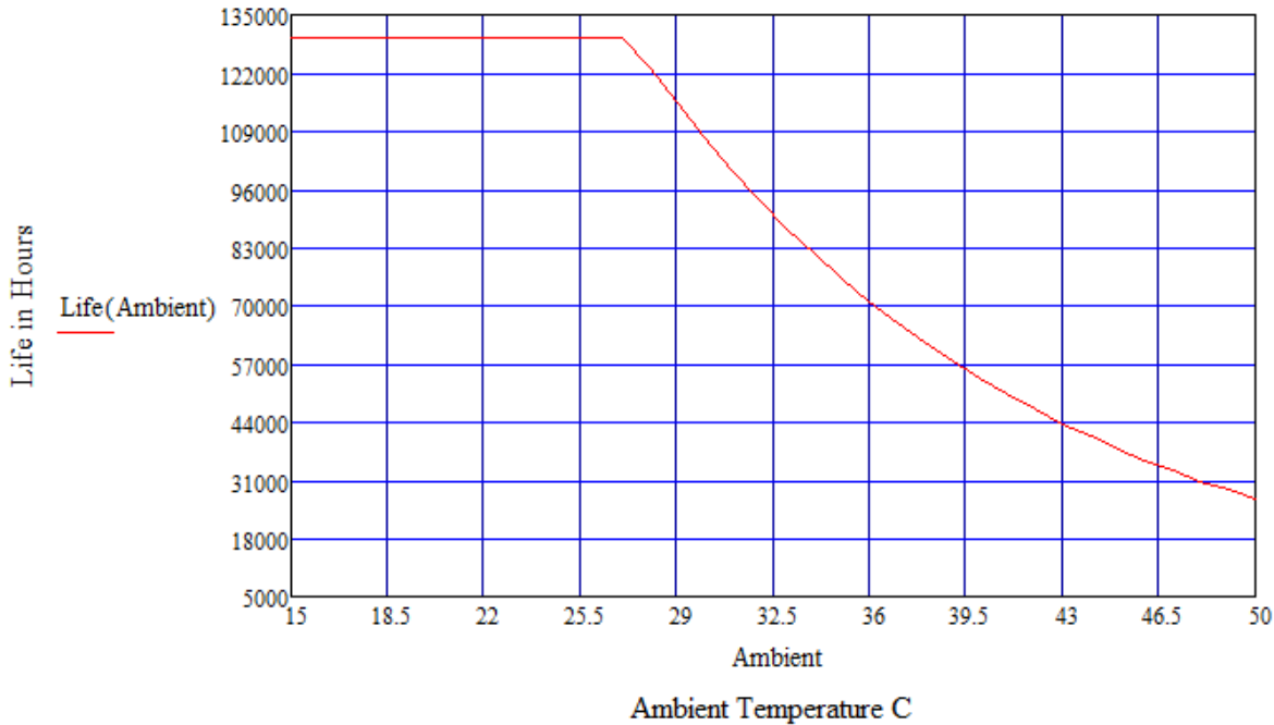
LPF300W-XX-PCXXX-RD Estimated Life Full Load @ 120Vac
