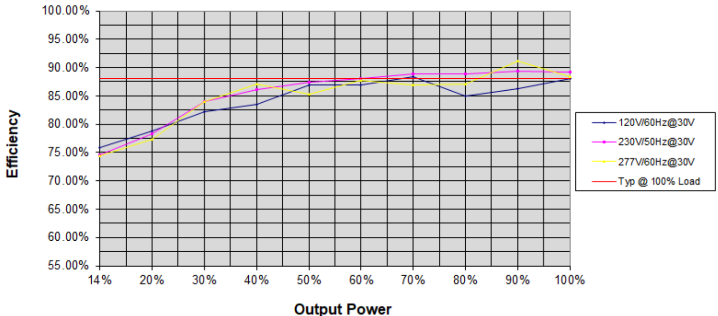
Efficiency vs. Output Power
