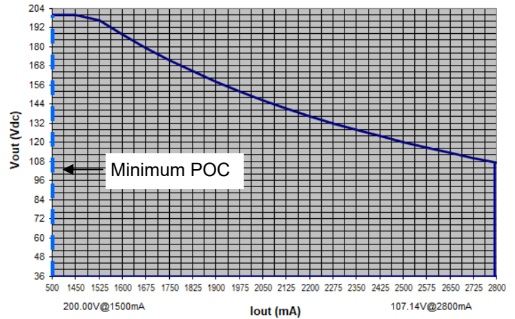
LPF300W-200-PC2800-RD OPERATING WINDOW Vout (Vdc) vs. Output Current (mA)
