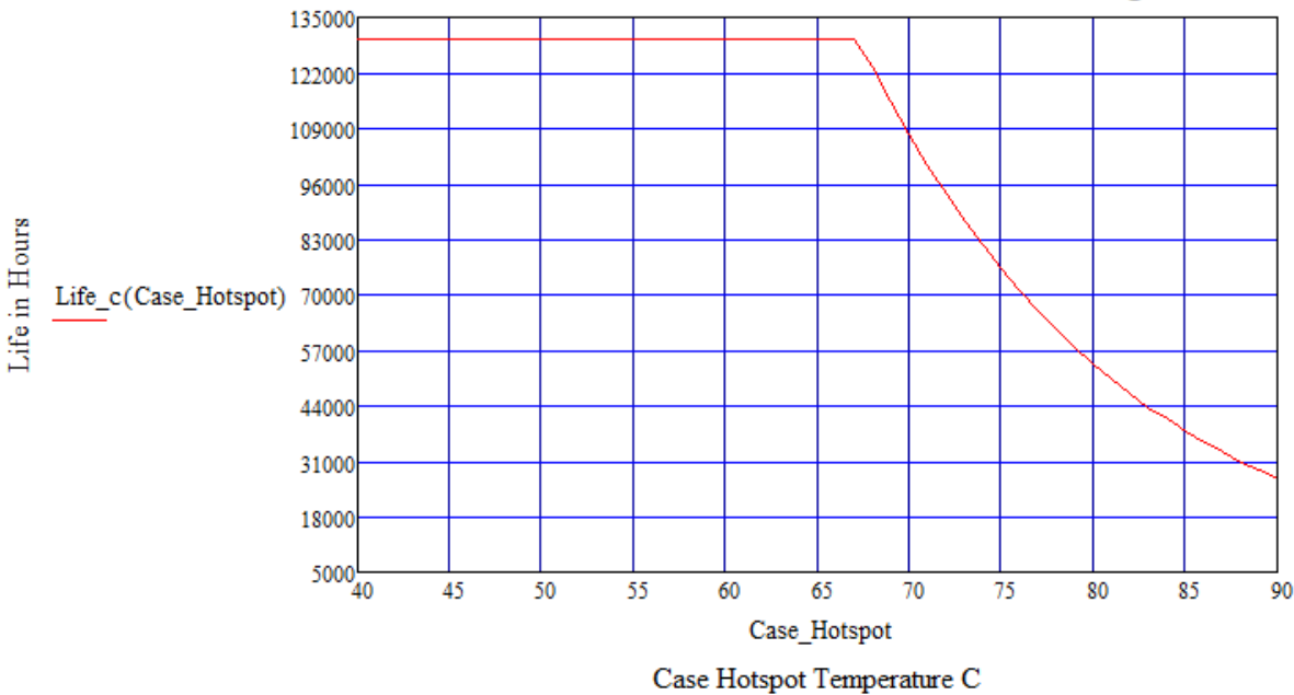
LPF300W-XX-PCXXX-RD Estimated Life Full Load @ 120Vac
