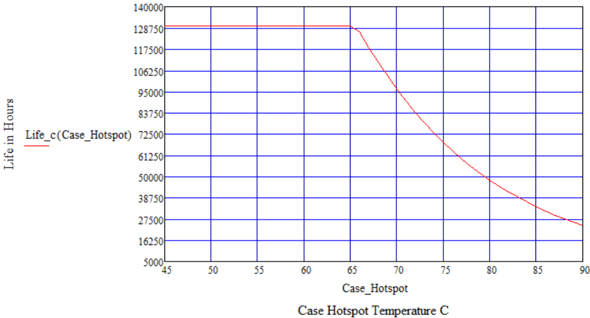
LPF40W Estimated Life Full Load @ 120Vac
