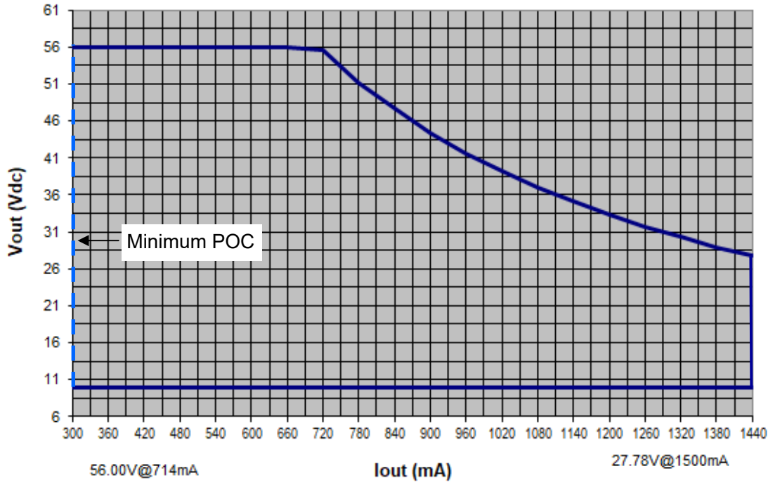
LPF40W-56-PC1500-RD OPERATING WINDOW Vout (Vdc) vs. Output Current (mA)
