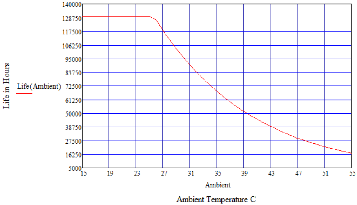
LPF40W Estimated Life Full Load @ 120Vac
