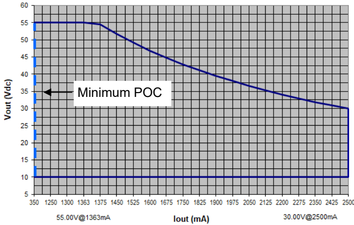
LPF75W-55-PC2500-RD OPERATING WINDOW Vout (Vdc) vs. Output Current (mA)
