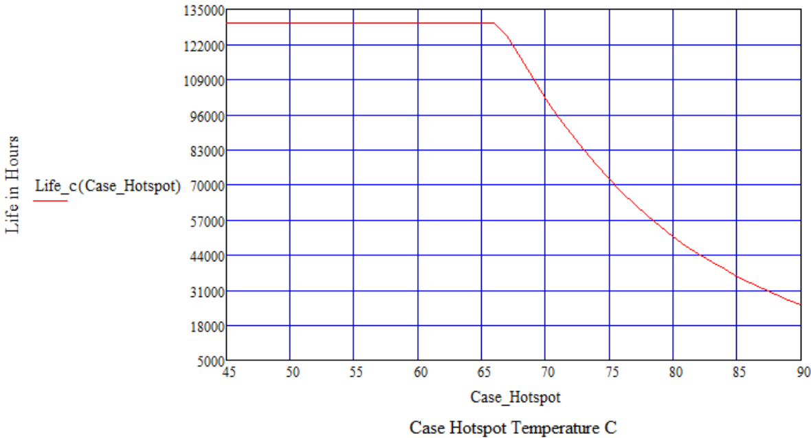
LPF75W-XX-PCXXX-RD Estimated Life Full Load @ 120Vac
