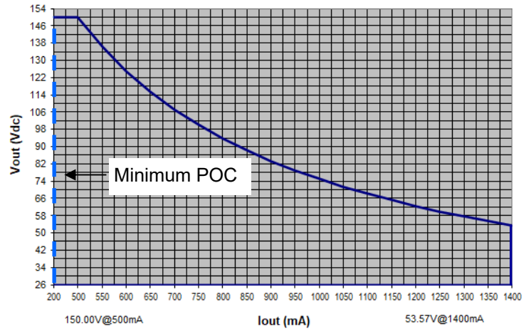
LPF75W-150-PC1400-RD OPERATING WINDOW Vout (Vdc) vs. Output Current (mA)
