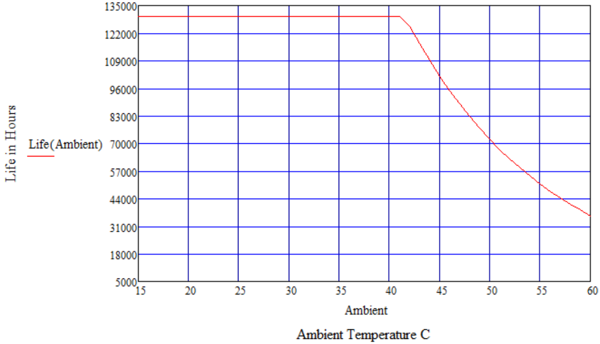
LPF75W-XX-PCXXX-RD Estimated Life Full Load @ 120Vac
